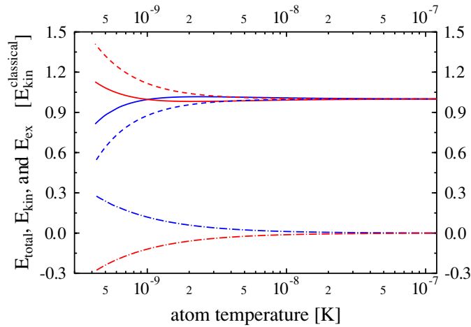
Figure 2. Total (solid), kinetic (dashed), and exchange (dash-dotted) energies of a potassium gas with n = 10^9 \text{cm}^{-3} normalized by the kinetic energy of the corresponding classical system. Interactions are modelled by the Morse potential (7). The blue and red lines correspond to bosonic ( ^{39}\text{K} ) and fermionic ( ^{40}\text{K} ) atoms, respectively.
